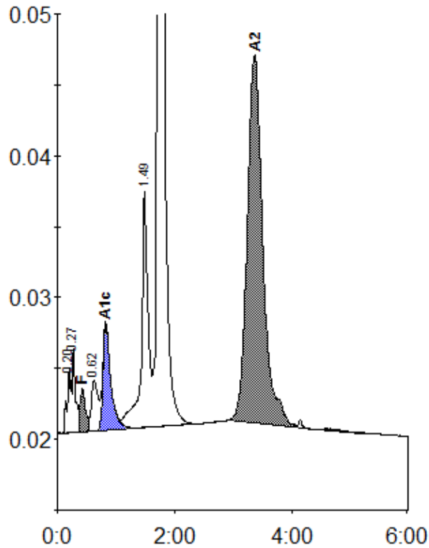
Peak table - ID: 11571443
