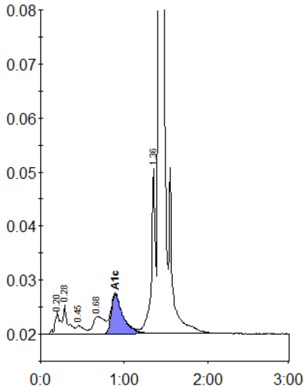
Peak table - ID: 11505278
