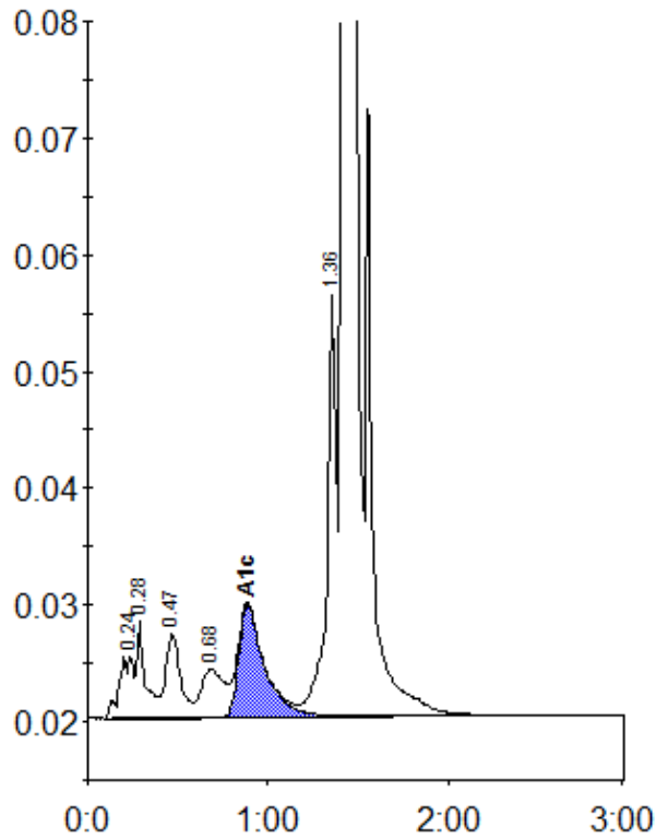
Peak table - ID: 11500778
