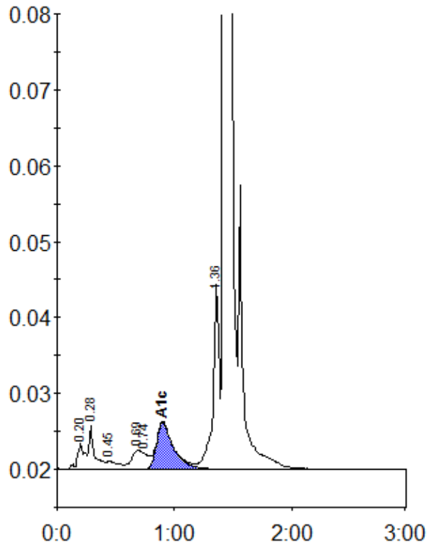
Peak table - ID: 11056669
