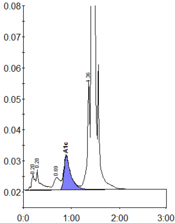
Peak table - ID: 11056670
