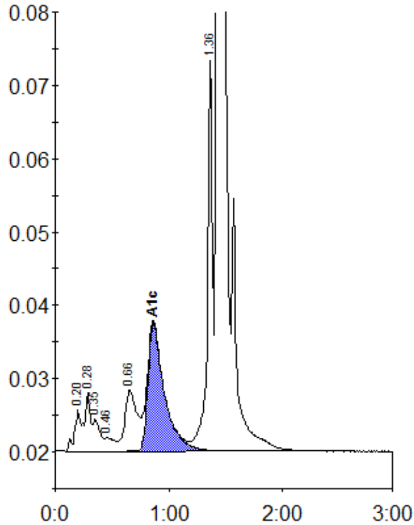
Peak table - ID: 11490733
