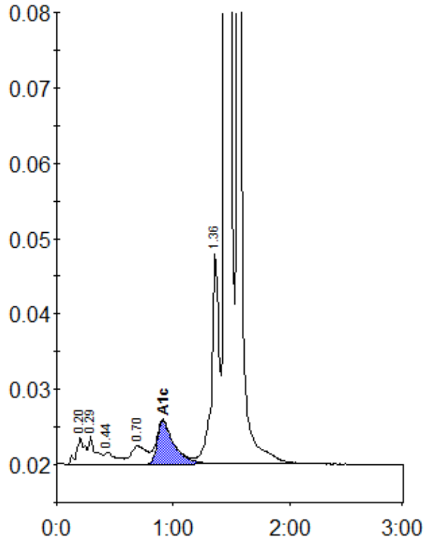
Peak table - ID: 11516089
