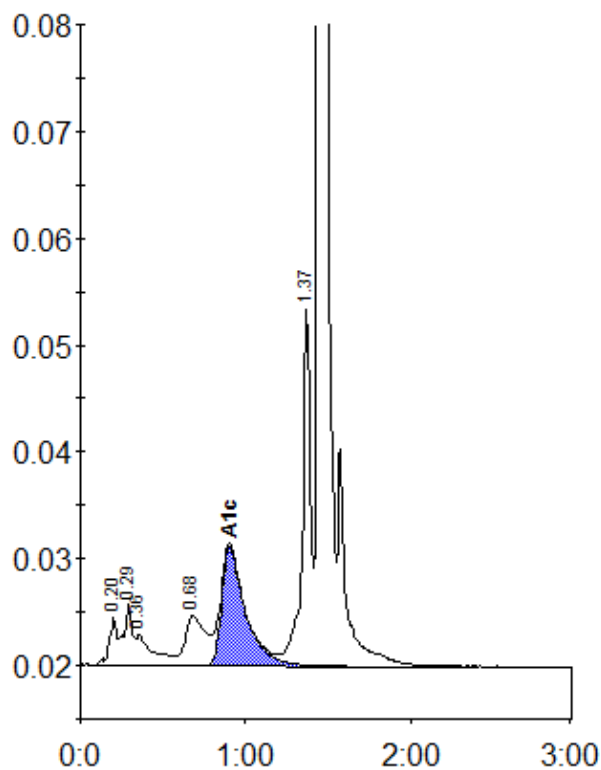
Peak table - ID: 11462044
