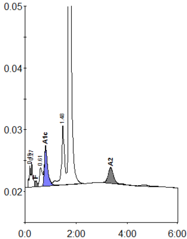
Peak table - ID: 11458009
