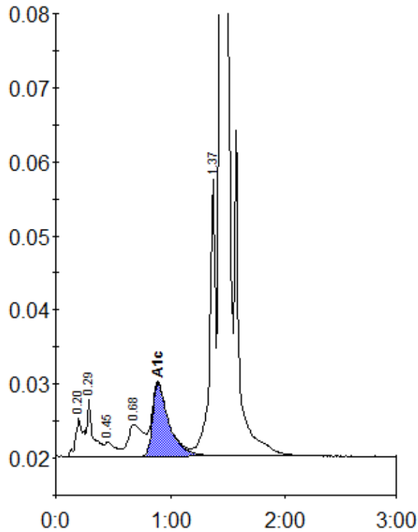
Peak table - ID: 11497674
