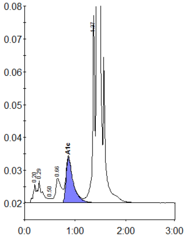
Peak table - ID: 11529167
