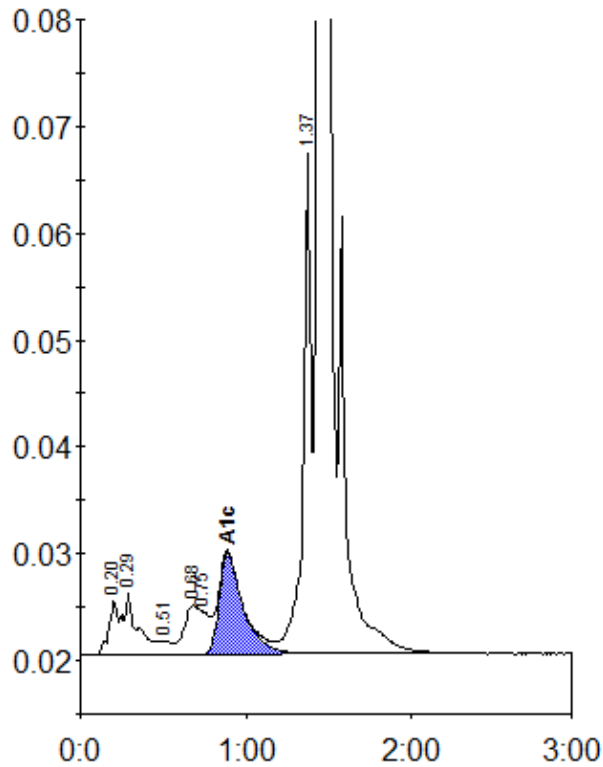
Peak table - ID: 11353495
