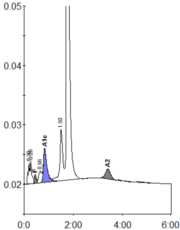
Peak table - ID: 024334522
