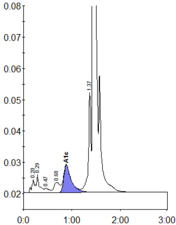
Peak table - ID: 11399107
