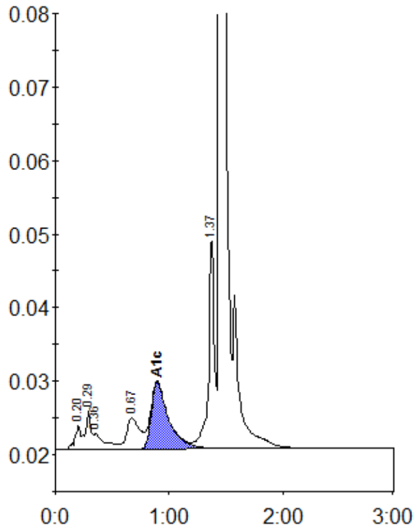
Peak table - ID: 11446945
