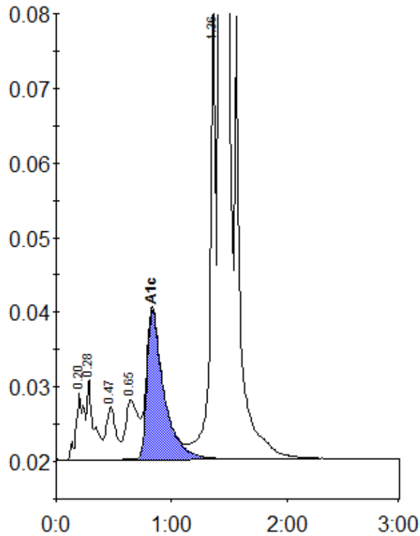
Peak table - ID: 11621983
