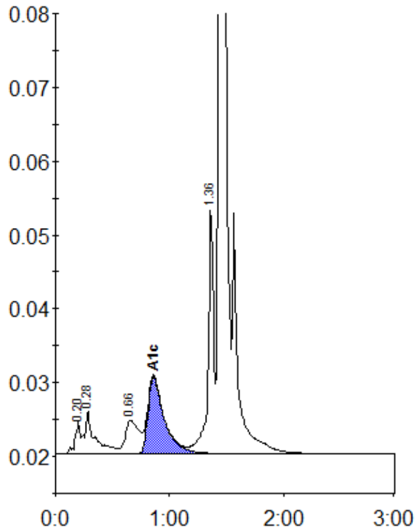
Peak table - ID: 11559431
