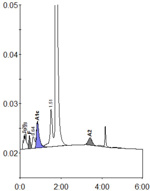
Peak table - ID: 11525312
