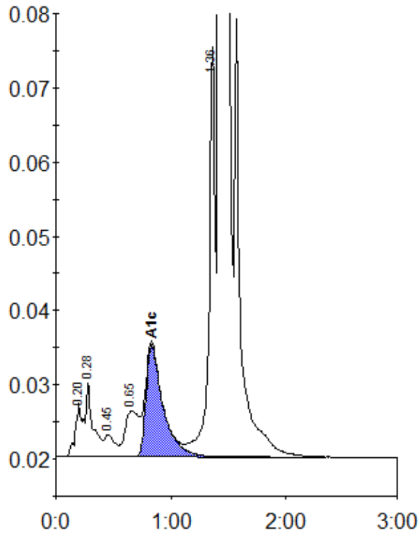
Peak table - ID: 11557531
