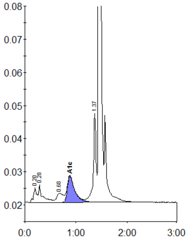
Peak table - ID: 11525569
