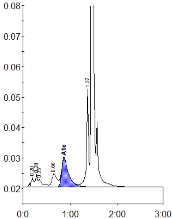
Peak table - ID: 11515991
