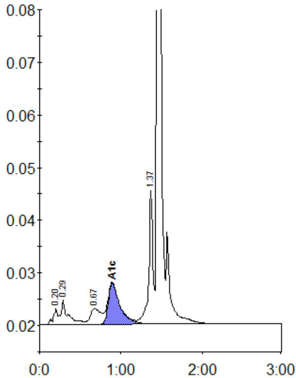
Peak table - ID: 11447858
