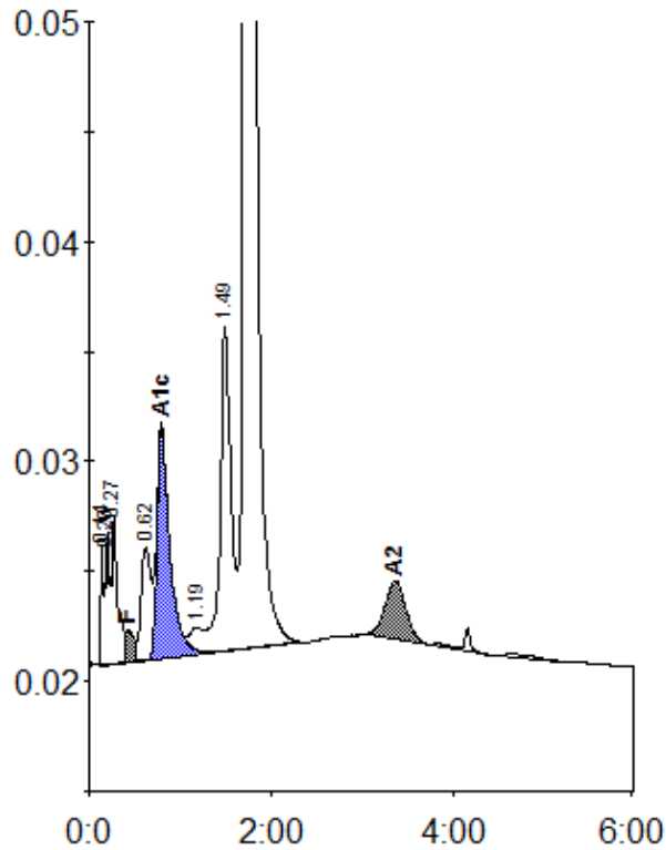
Peak table - ID: 11245853
