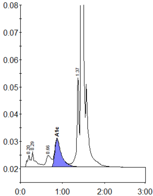
Peak table - ID: 11501332
