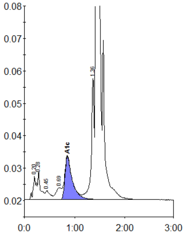
Peak table - ID: 11589946
