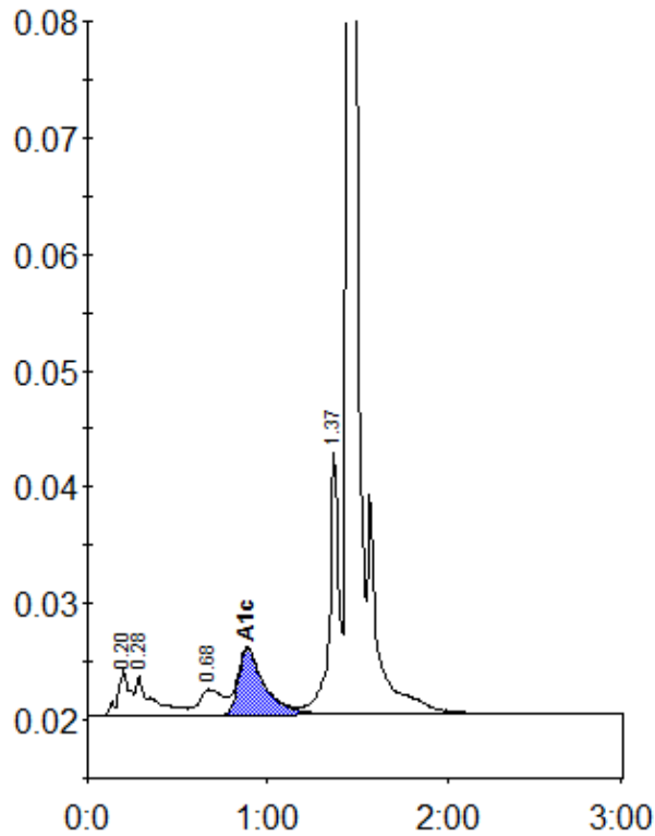
Peak table - ID: 11586276
