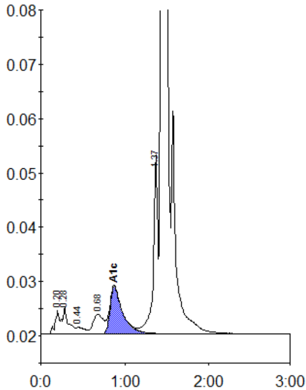
Peak table - ID: 11565292
