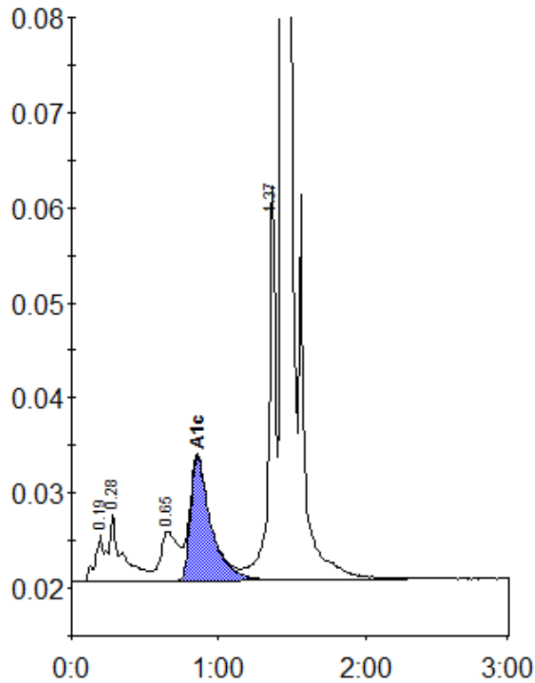
Peak table - ID: 11532052
