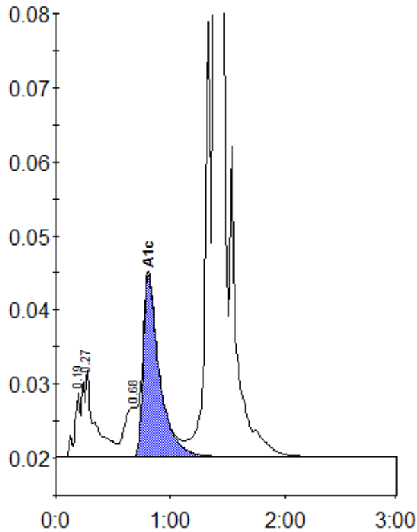
Peak table - ID: 11268351
