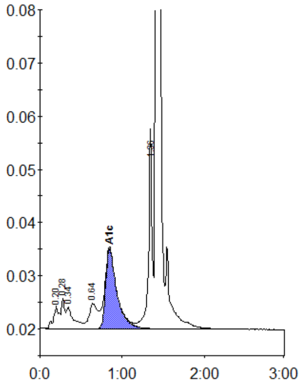
Peak table - ID: 11462618
