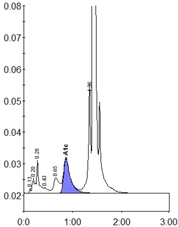
Peak table - ID: 11631143
