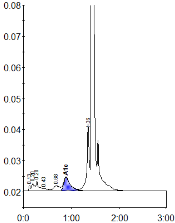
Peak table - ID: 11573016
