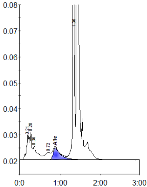
Peak table - ID: 11565853
