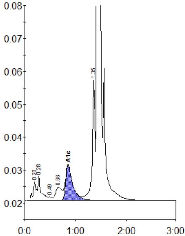
Peak table - ID: 11581443
