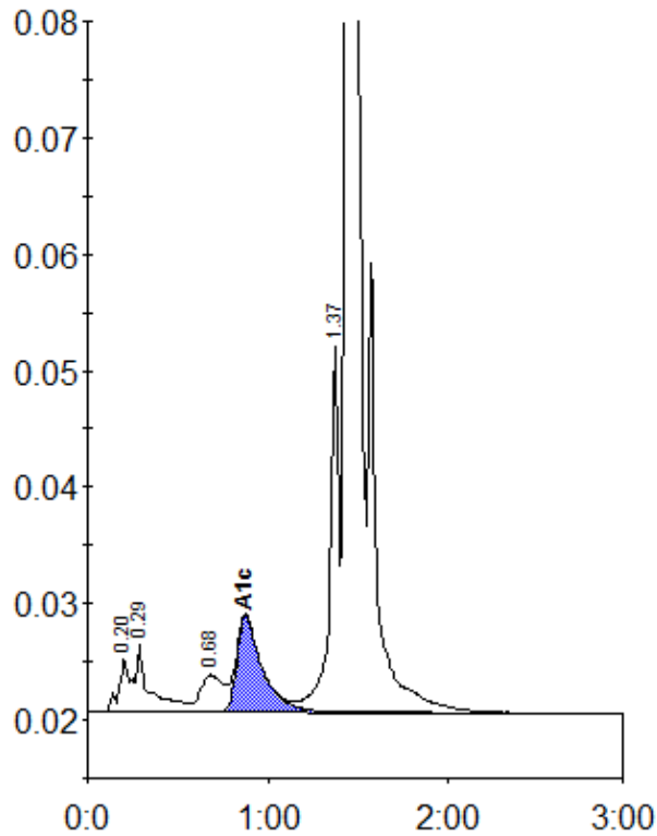
Peak table - ID: 11575463
