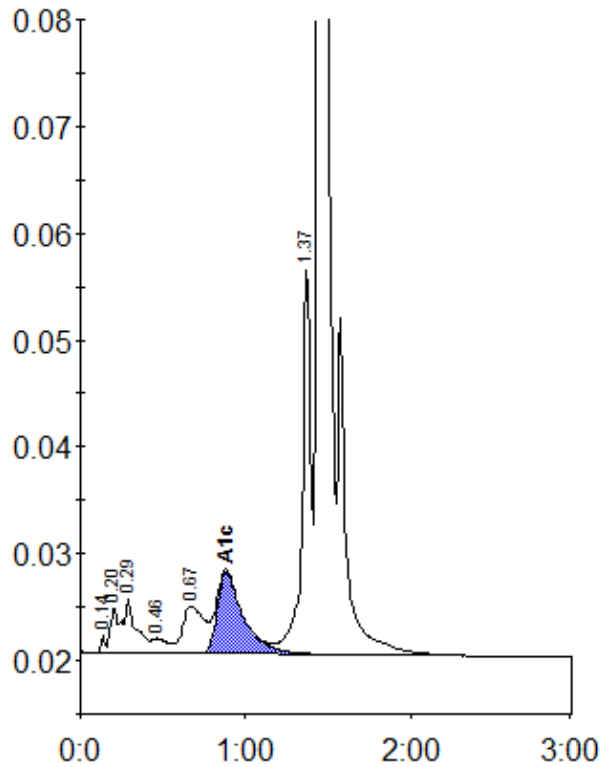
Peak table - ID: 11574103
