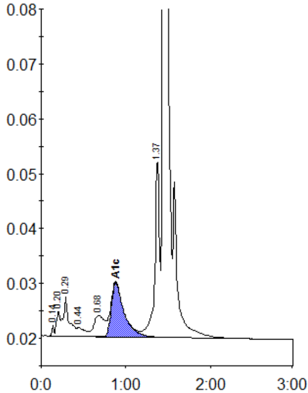
Peak table - ID: 11550206
