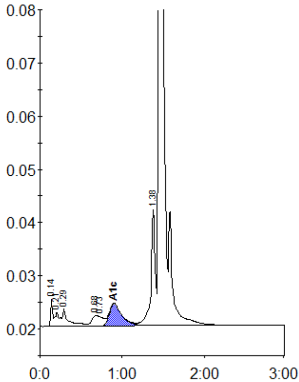
Peak table - ID: 11271566
