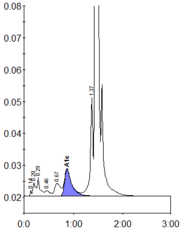
Peak table - ID: 11550438
