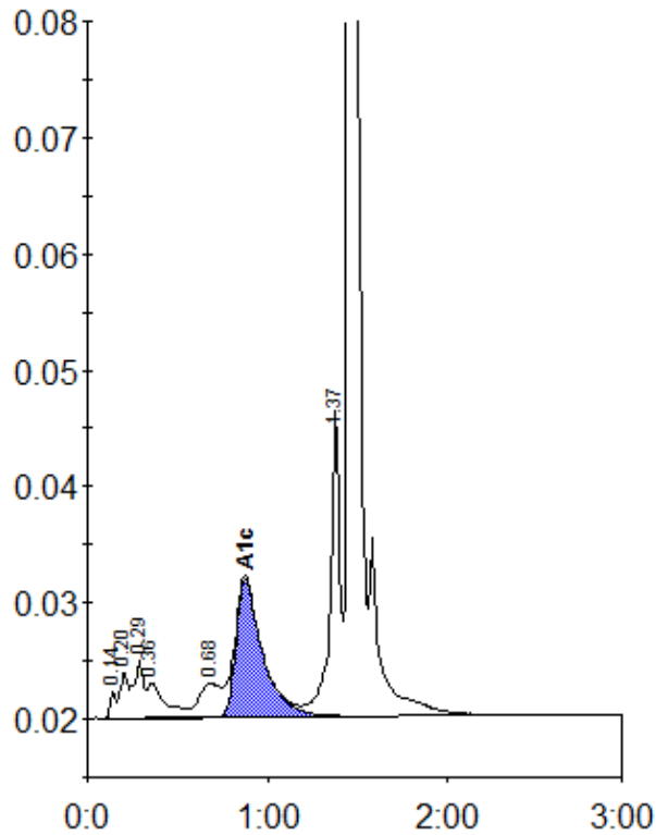
Peak table - ID: 11578014
