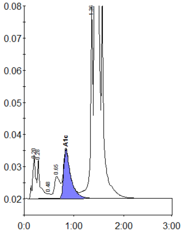
Peak table - ID: 11619590
