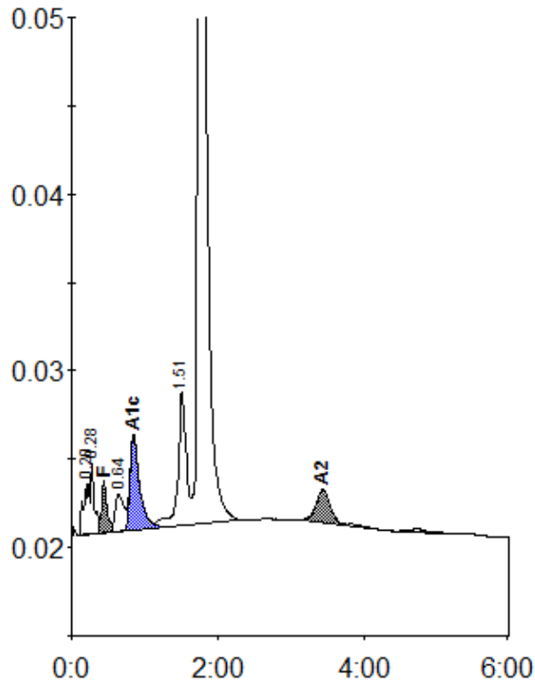
Peak table - ID: 11588203
