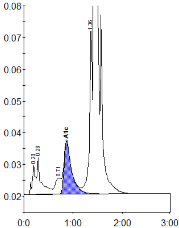
Peak table - ID: 11552171
