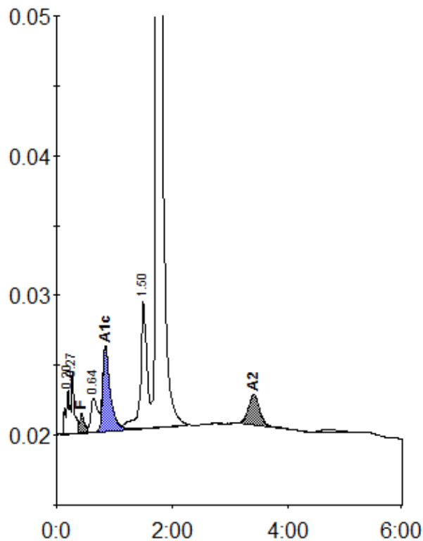
Peak table - ID: 11593217
