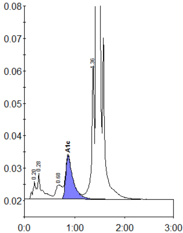
Peak table - ID: 11590594
