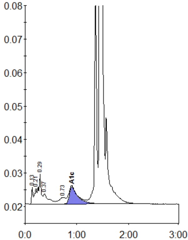
Peak table - ID: 11392612
