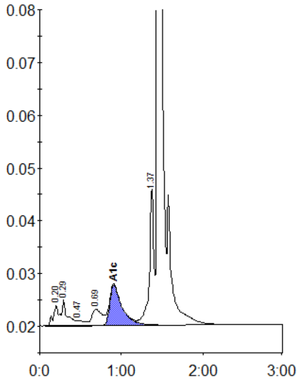
Peak table - ID: 11588496
