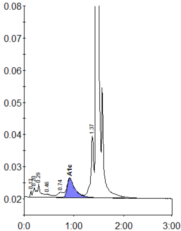
Peak table - ID: 11567388
