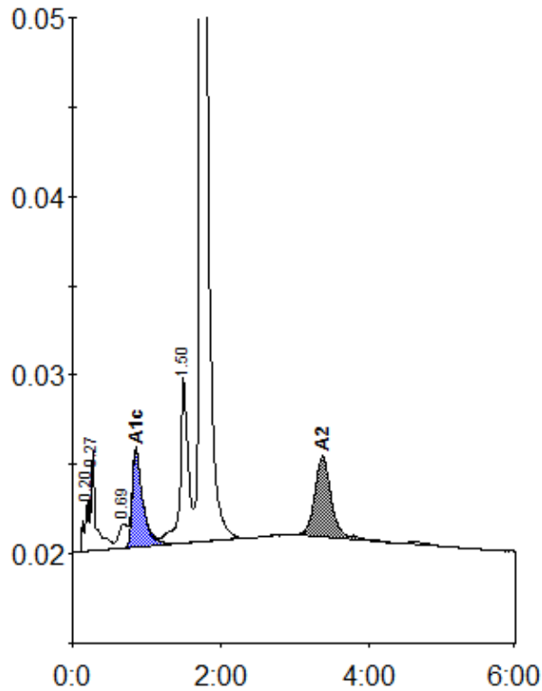
Peak table - ID: 11619180
