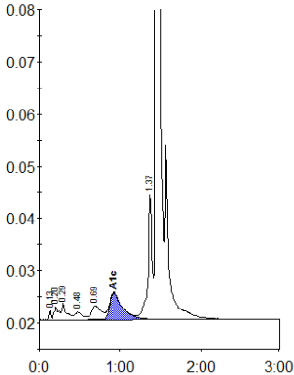
Peak table - ID: 11588973
